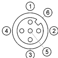
Presca M12: Ethernet
