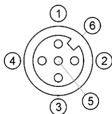
Presa M12: Telecamera
